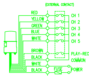
ELECTRICAL CONNECTION DIAGRAM
